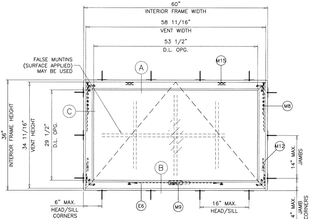
TYPICAL ELEVATION
