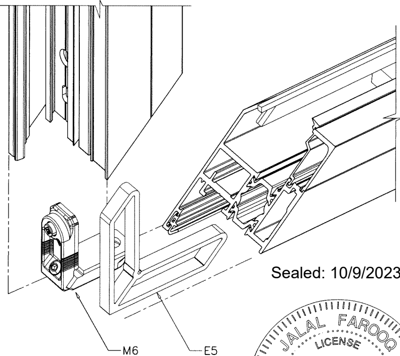
VENT ASSEMBLY
